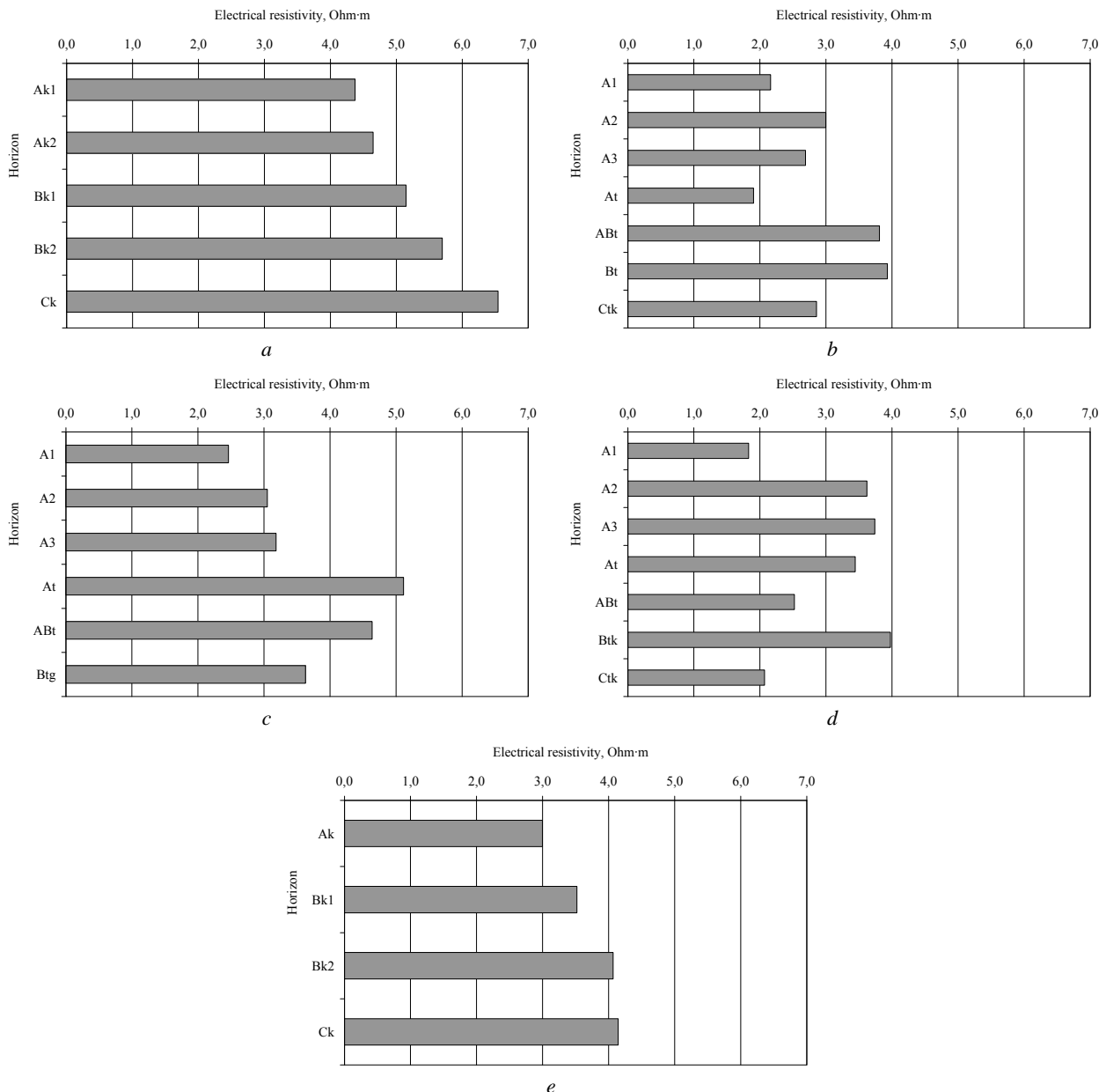
Fig. 1. Electrical resistance of the studied soils: a – trial plot 1; b – trial plot 2; c – trial plot 3; d – trial plot 4; e – trial plot 5
