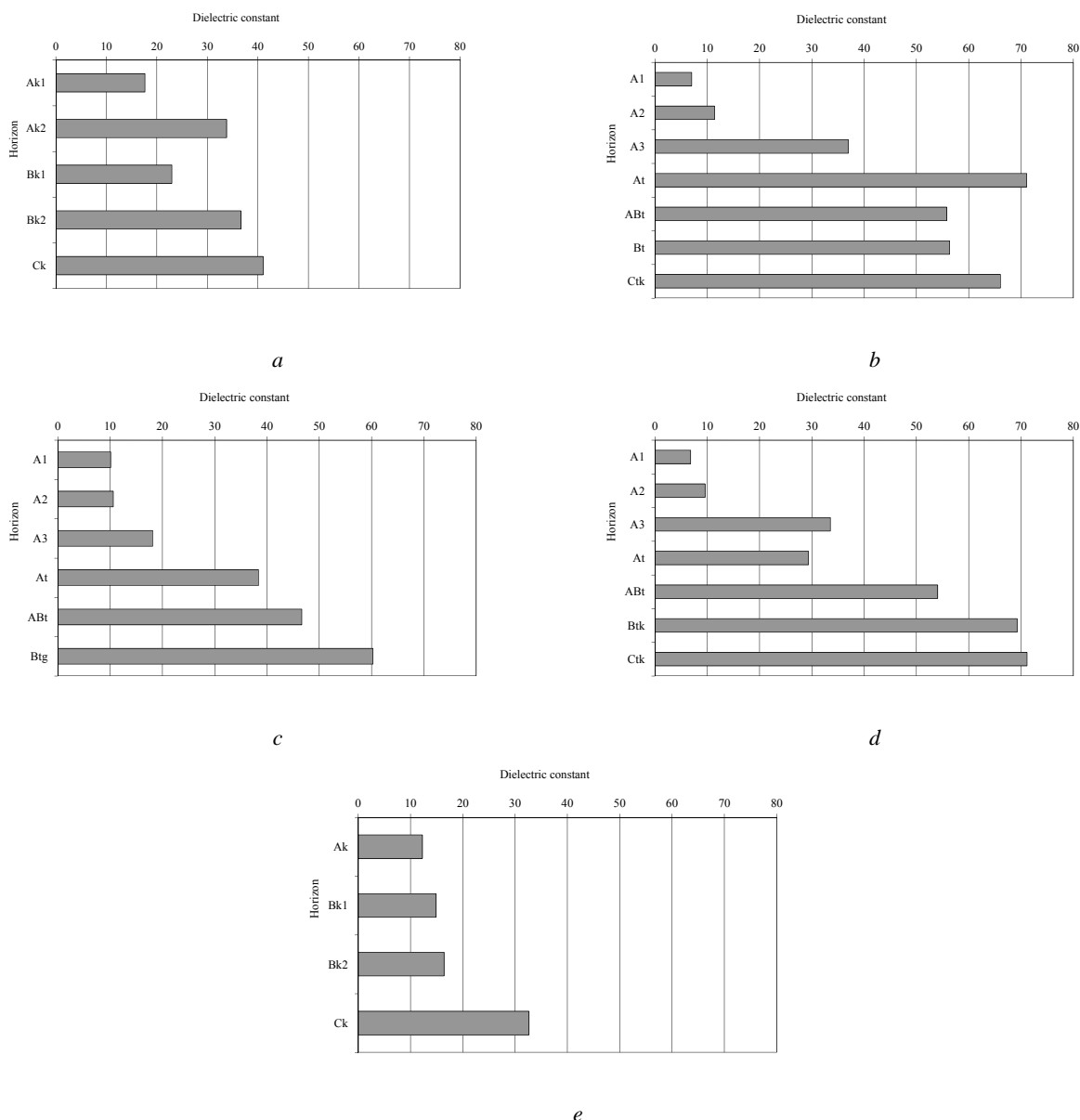
Fig. 2. Dielectric constant of the studied soils: a – trial plot 1; b – trial plot 2; c – trial plot 3; d – trial plot 4; e – trial plot 5
